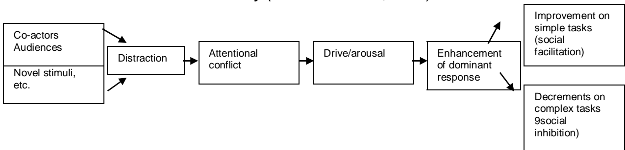
Schema 2. Distraction conflict theory (based on Baron, 1986).
