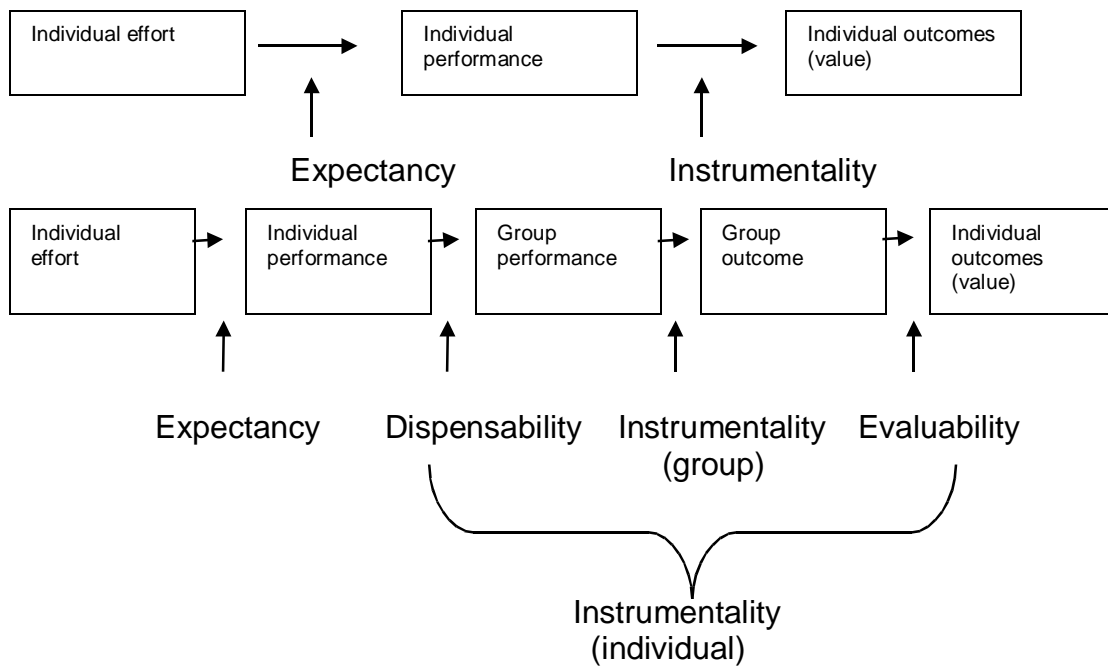
Schema 3. Expectancy-value theory for individuals and group members:
