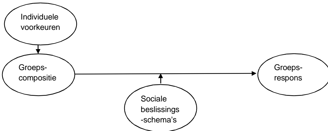
Schema 4. Social decision scheme theory, Davis (1973)
